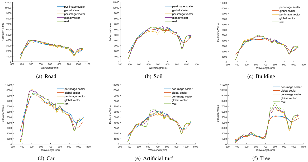
Fig. 8. Comparison of generated spectra by different t learning strategies. “per-image scalar” means t is a trainable scalar and is optimized separately for every image. “global scalar” means t is a trainable scalar and is optimized as a global variable on the whole dataset. “per-image vector” means t is a trainable scalar and is optimized separately for every image. “global vector” means t is a trainable vector and is optimized as a global variable on the whole dataset (our final implementation).
