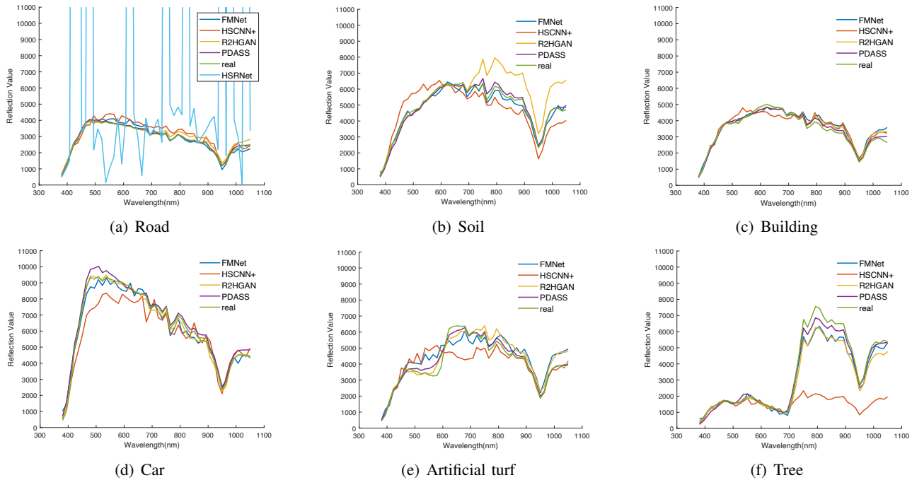
Fig. 6. Spectral curves generated by different methods: HSRNet [61], HSCNN+ [71], FMNet [15], R2HGAN [20], and PDASS (ours). Because HSRNet has a numerical overflow problem, we only visualize its result in the first sub-figure for easy comparison.
