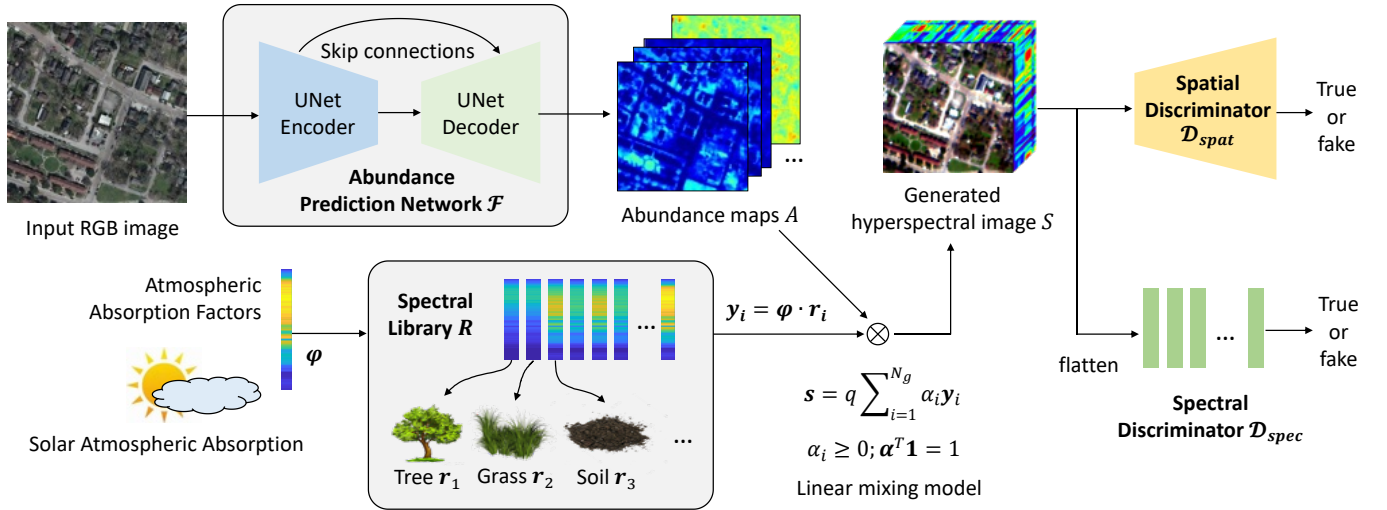
Fig. 2. An overview of the proposed method. Given an input RGB image, we introduce a U-Net based abundance prediction network to generate pixel-wise spectral abundance maps. With a spectral library and linear mixing model, the hyperspectral image can be constructed. We also introduce a spatial discriminator and a spectral discriminator to improve the realism and visual quality of the generated hyperspectral image. All networks can be trained in an end-to-end fashion with self-supervised reconstruction losses.
