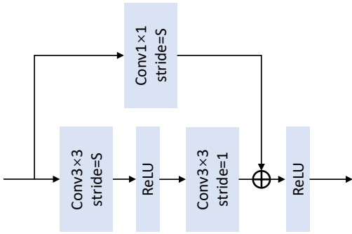
Fig. 3. Structure of resblocks in our abundance prediction network.
