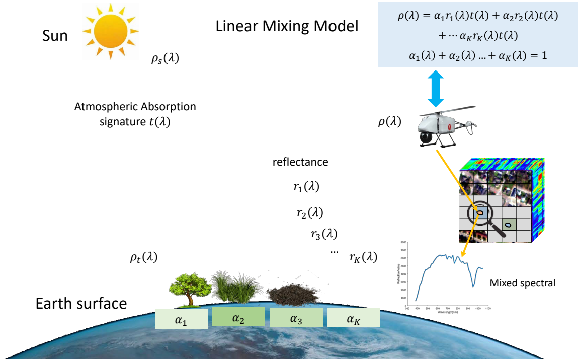
Fig. 1. Hyperspectral remote sensing imaging model. The sunlight \rho_s(\lambda) passes through the atmospheric absorption t(\lambda) and incidents to the ground \rho_t(\lambda) . Reflectance of different ground objects are represented as r_1(\lambda), r_2(\lambda), \dots and their abundance in pixel area is represented as \alpha_1, \alpha_2, \dots . Finally, the sensor receives the reflected spectra and the spectral image is obtained according to the Linear Mixing Model.
