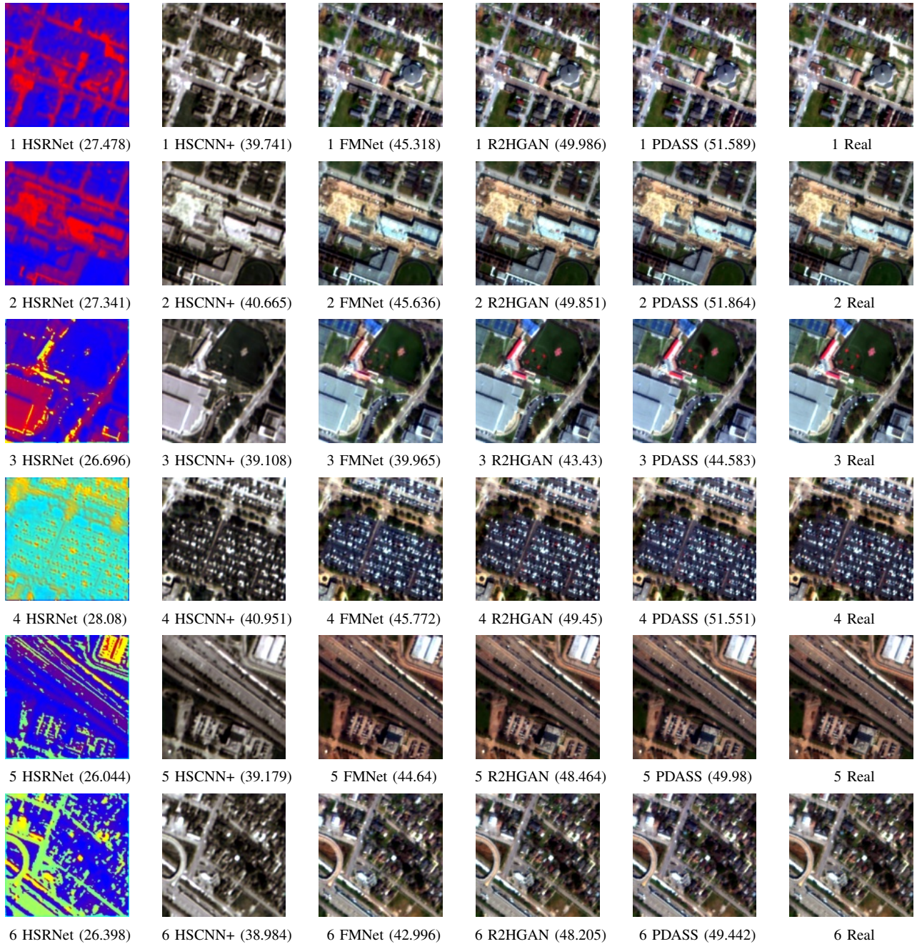
Fig. 4. False-color visualization (band No. 23, 12, and 5) of the generated hyperspectral image with different methods: HSRNet [61], HSCNN+ [71], FMNet [15], R2HGAN [20], and PDASS (ours). The test image ID and reconstruction MPSNR are also given. For example, 1 HSRNet (27.478) means the result of HSRNet on test image #1 with MPSNR = 27.478.
