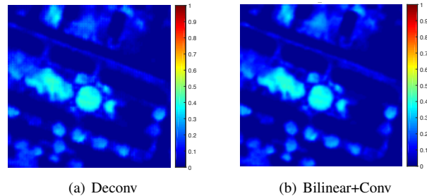
Fig. 9. Abundance maps (“Lawn_Grass”) generated by \mathcal{F} under two upsampling configurations: (a) deconvolution, and (b) bilinear upsampling + convolution. There is a noticeable checkerboard artifact produced by the deconvolution layers.
