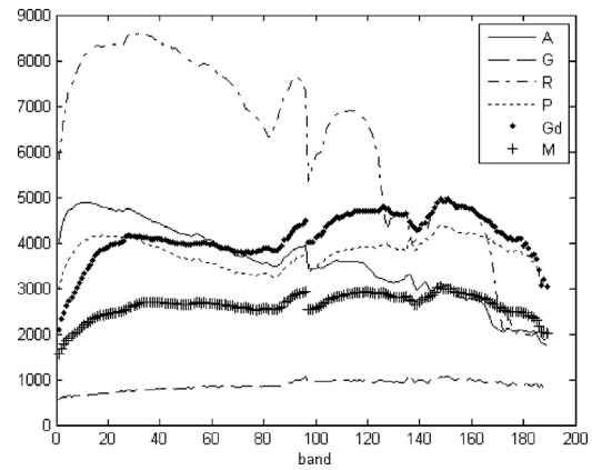
Fig. 1. Spectra of A, G, R, P, Gd and M.
