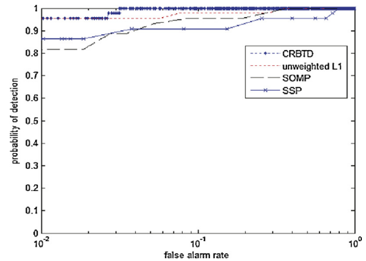
Fig. 6. The ROC curves of CRBTD, SOMP, SSP and unweighted \ell_1 method in AVIRIS-I HSI.
